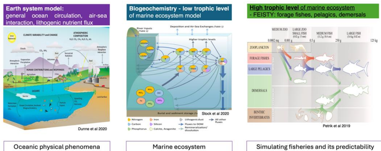
Fig.1. Research outlook for marine ecosystem predictability with earth system model (Dunne et al 2020), marine biogeochemistry (Stock et al 2020), and high trophic level of marine ecosystem (Petrik et al 2019)
