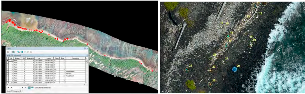
Fig. 2 A swath of Kaua'i coastline in ArcGIS and the data table of the identified dots of debris (left), with a zoomed screenshot of identified marine debris with numbers on Kamilo Point, Hawaii Island (right).
